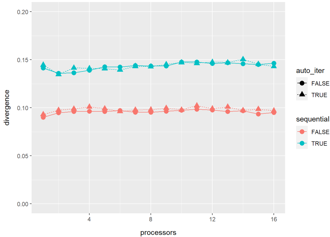
Figure 3: The average Jansen-Shannon divergence of the \phi parameter. Sequential classification is enabled when “sequential” is true (blue). Convergence detection is enabled when “auto_iter” is true (triangles). Divergence is computed by repeating the same model X times and comparing with the \phi parameter from the standard LDA model. The average divergence is computed by fitting the same model 10 times.
