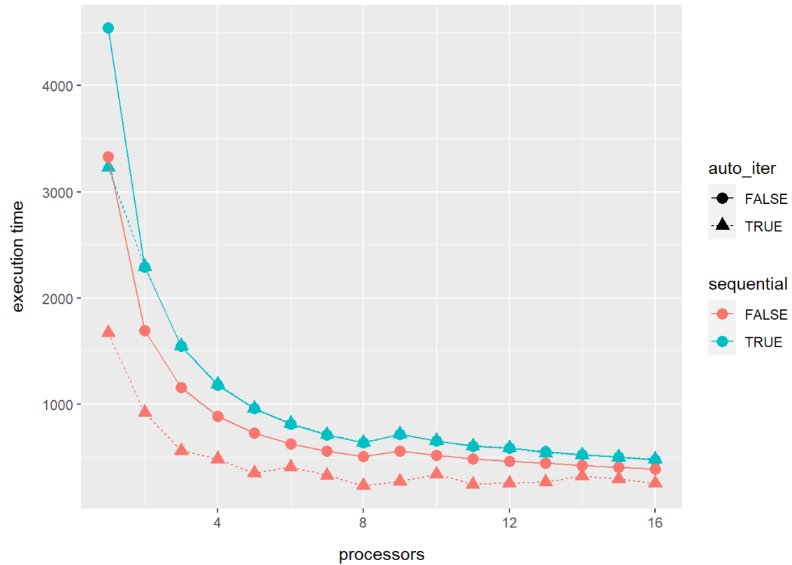
Figure 2: The average execution time for sequential and non-sequential models. Sequential classification is enabled when “sequential” is true (blue). Convergence detection is enabled when “auto_iter” is true (triangles). The average execution time is computed by fitting the same model 10 times.
